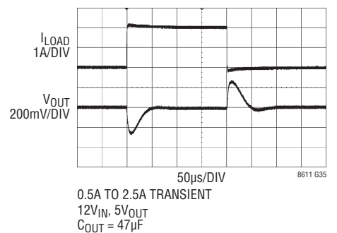
Transient Response
